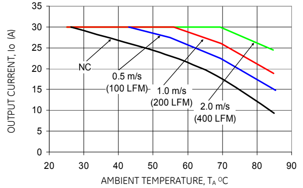
Figure 16. Derating Output Current versus Local Ambient Temperature and Airflow (direction shown in Figure 63).
