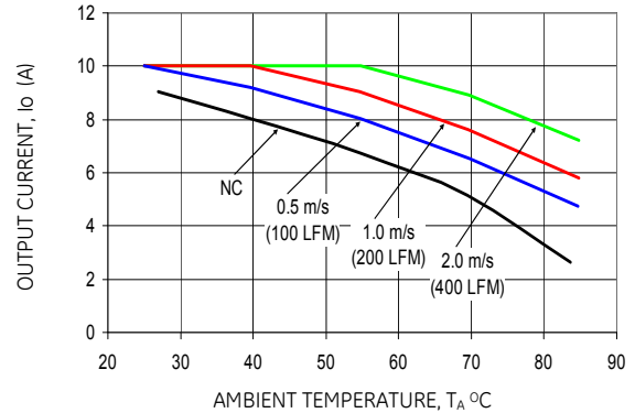
Figure 4. Derating Output Current versus Local Ambient Temperature and Airflow (direction shown in Figure 63).
