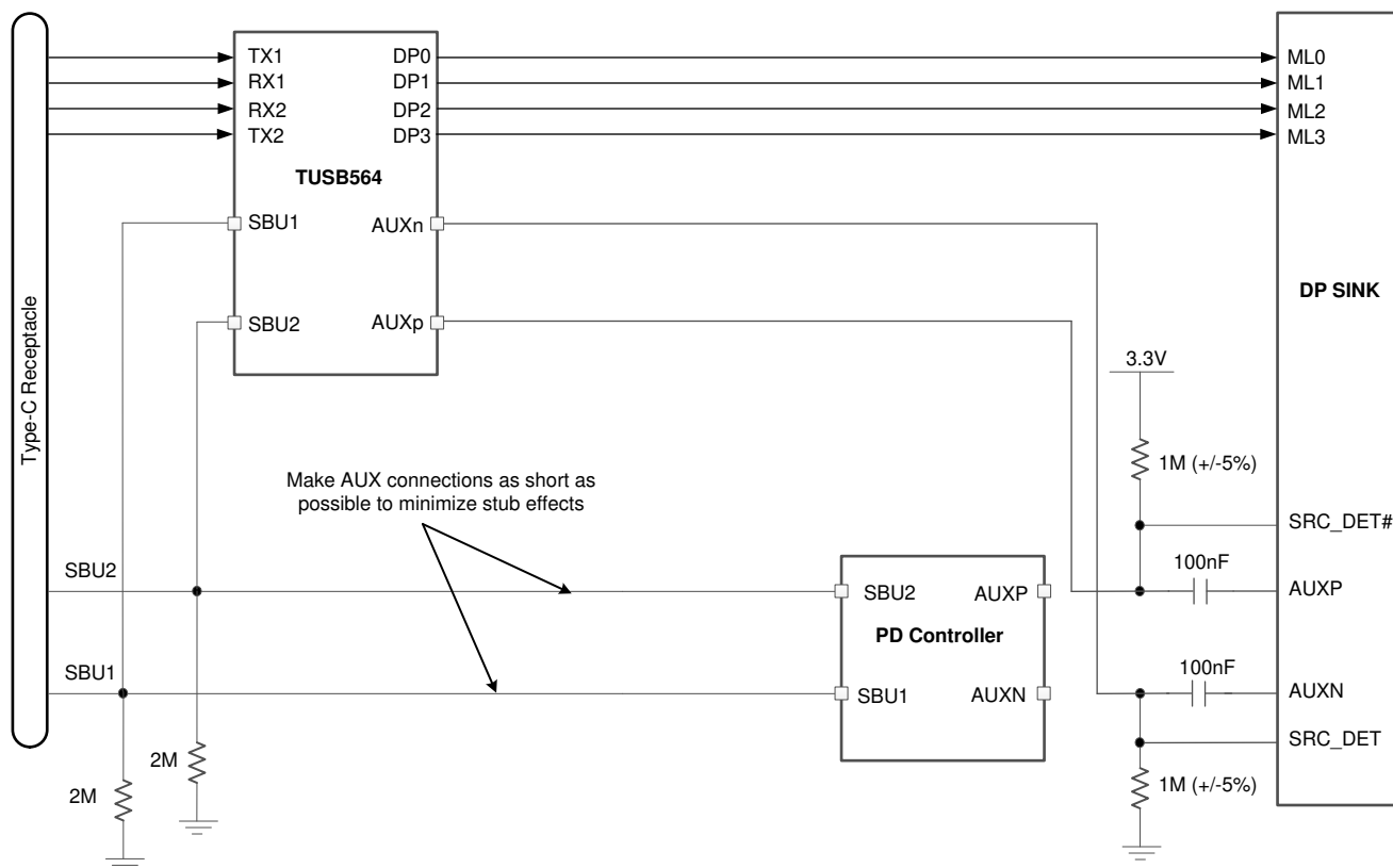
Figure 9-3. DisplayPort AUX Connections for UFP_D Pin Assignment E with Internal AUX Switching
