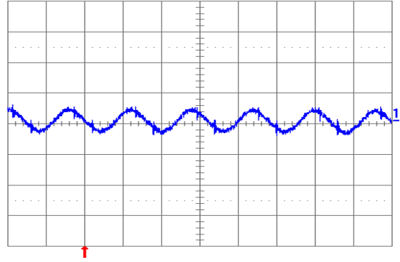
Fig. 3.3V.6: Output voltage ripple (20mV/div.) at full rated load current into a resistive load with external capacitance 100\mu F ceramic and V_{in} = 12V for V_{out} = 3.3V . Time scale: 2μs/div.
