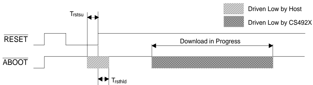
Figure 37. Autboot \overline{\text{INTREQ}} Behavior
