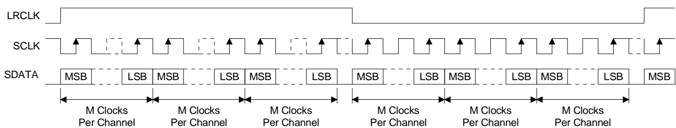
Figure 45. Multichannel Format
