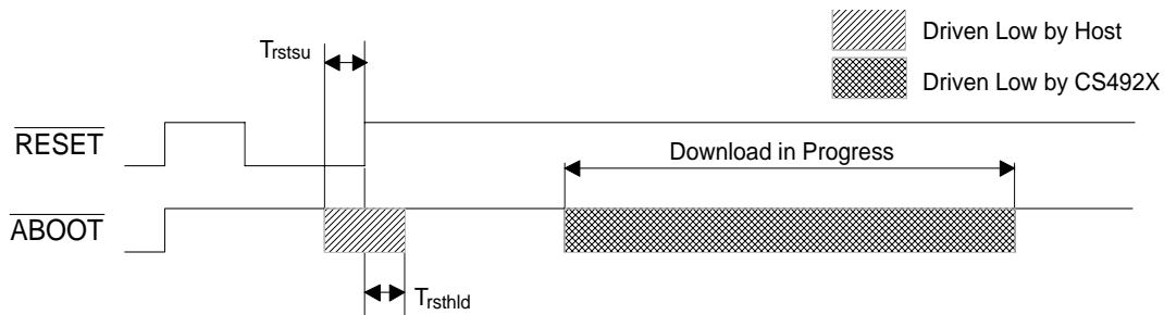
Figure 37. Autoboot \overline{\text{INTREQ}} Behavior
