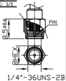
SMA(M) ST DETAIL : 'A' SCALE: 1/1
