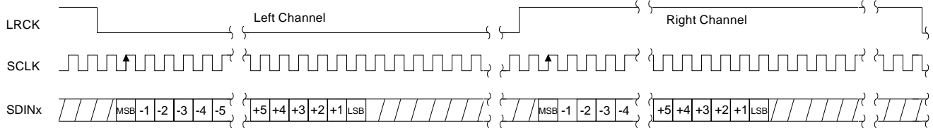
Figure 34. Format 1 - I²S up to 24-bit Data
