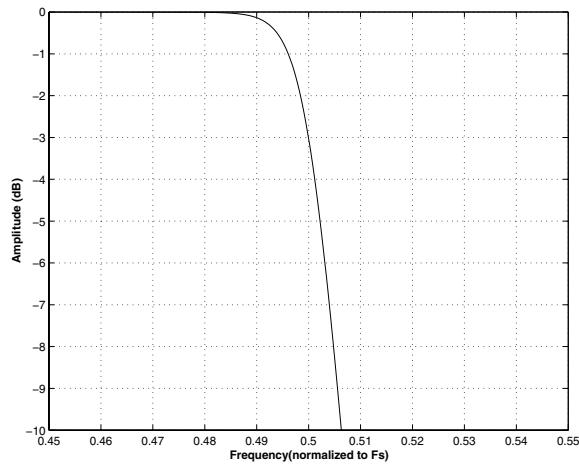
Figure 9. Single-Speed Transition Band (detail)
