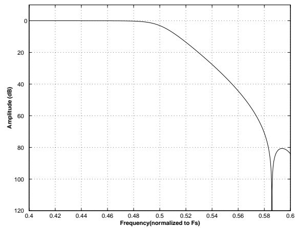
Figure 22. Double-Speed (fast) Transition Band
