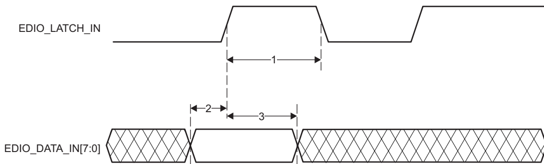
SPRS91x_TIMING_PRU_ECATCH_01
