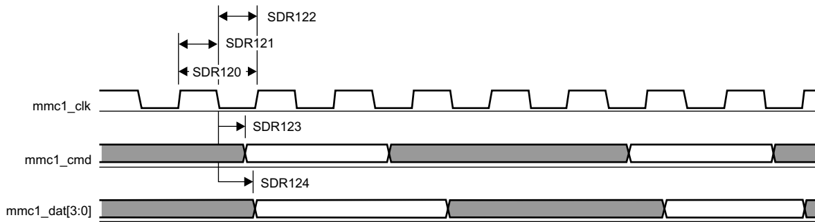
SPRS906_TIMING_MMC1_06
