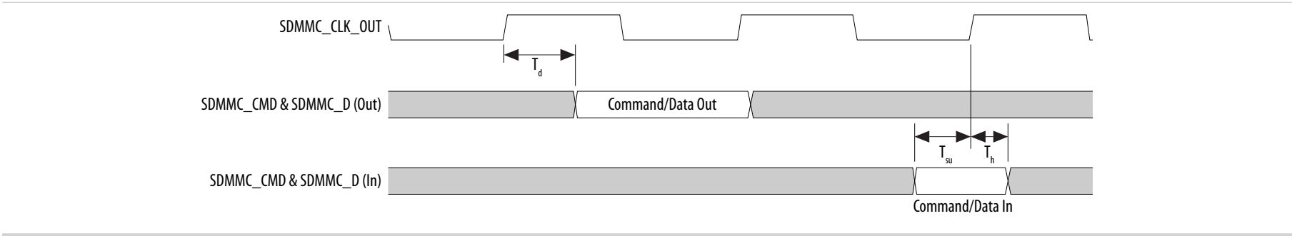
Figure 1-11: SD/MMC Timing Diagram
