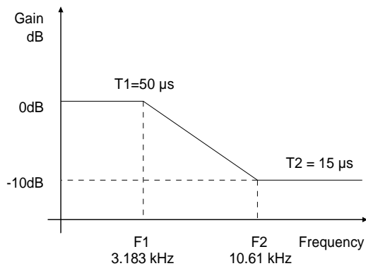
Figure 19. De-Emphasis Curve
