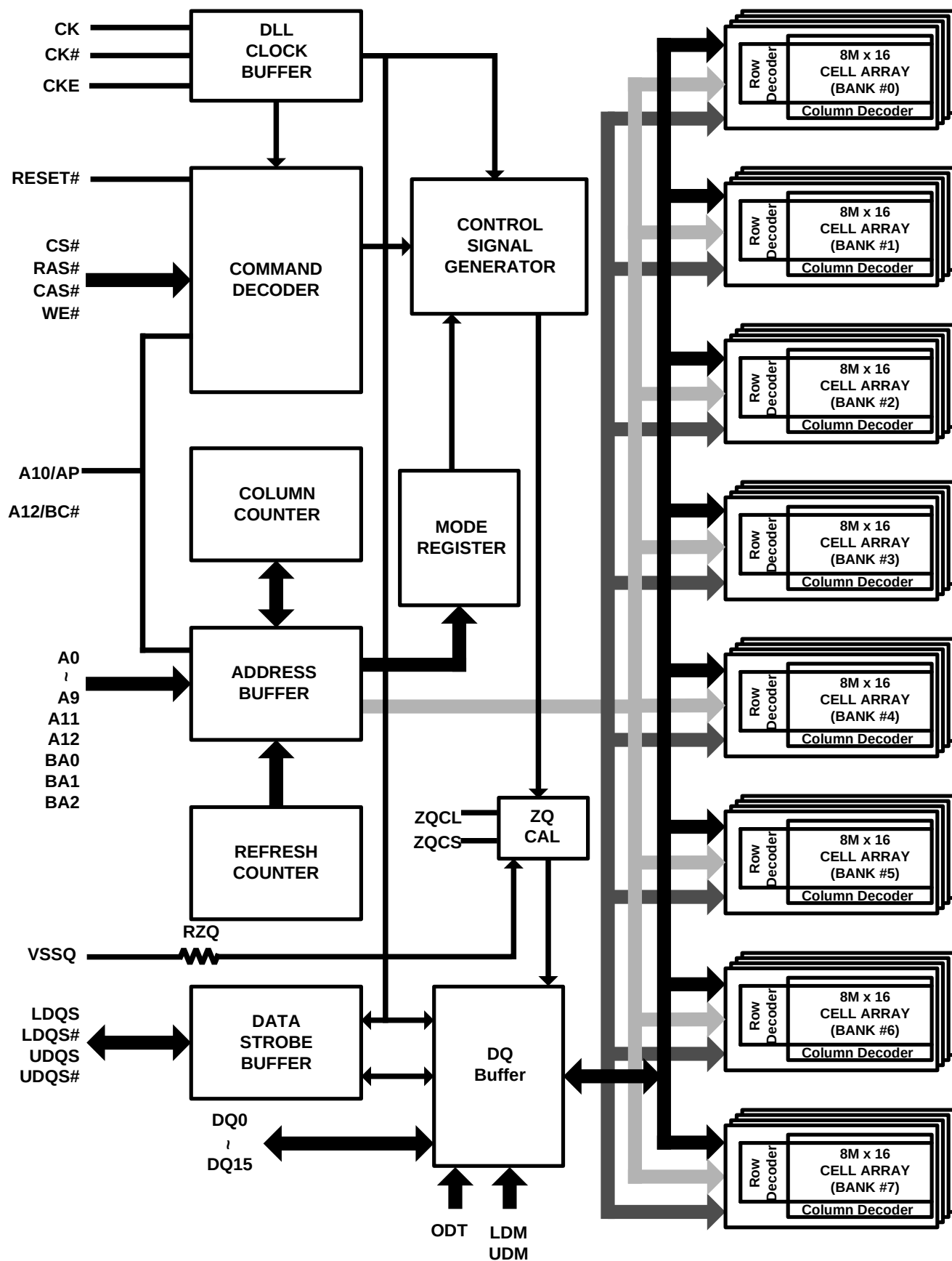
Figure 2. Block Diagram
