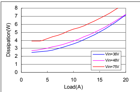
Fig. 15 Typical power dissipation curve of AVQ100B-48S05
