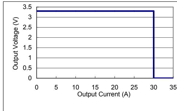
Fig. 9 Typical over-current of AVQ100B-48S3V3
