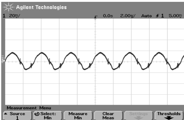
Fig. 18 Typical output ripple voltage AGQ100 -48S1V8, room temperature, I_o = I_{o,max}
