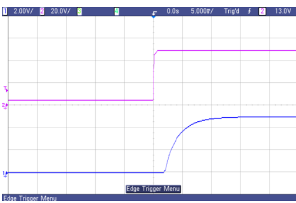
Fig.29 Typical start-up from power on of AVQ100B-48S05
