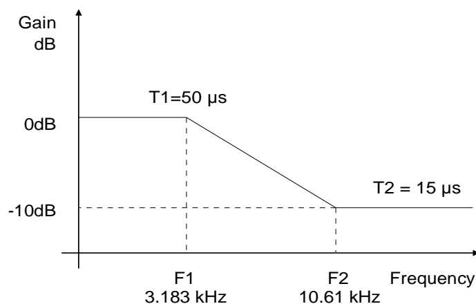
Figure 11. De-Emphasis Curve
