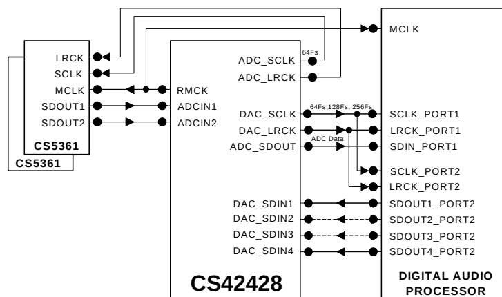
Figure 17. OLM Configuration #1
