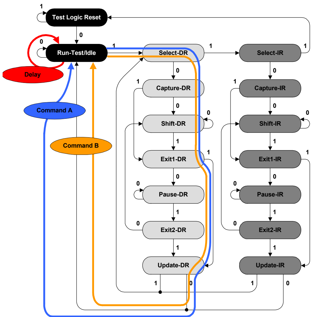
Figure 32: Inter-Command Delay
