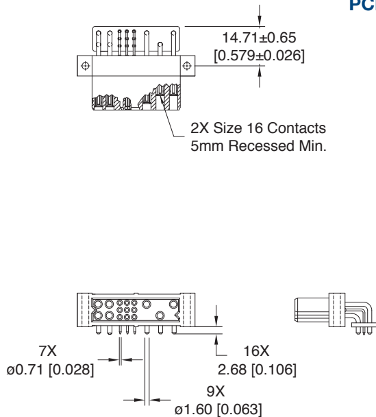
CONNECTOR DIMENSIONS
