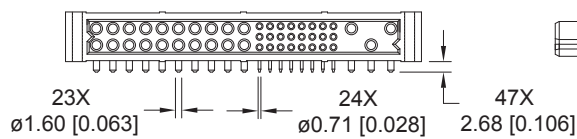
CONNECTOR DIMENSIONS
