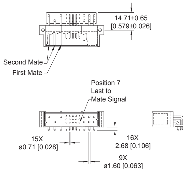
CONNECTOR DIMENSIONS
