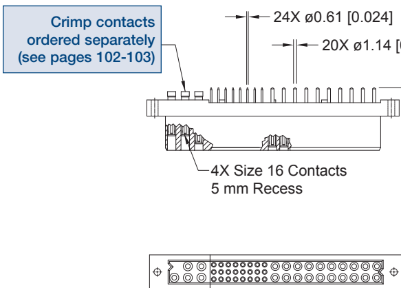
CONNECTOR DIMENSIONS
