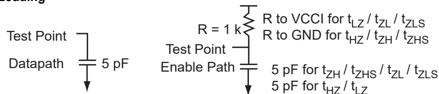
Figure 17 • AC Loading
