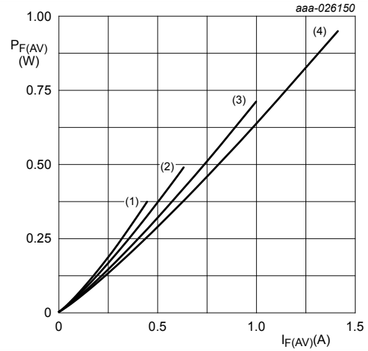
Fig. 6. Average forward power dissipation as a function of average forward current; typical values T_j = 150\text{ °C} (1) \delta = 0.1 (2) \delta = 0.2 (3) \delta = 0.5 (4) \delta = 1
