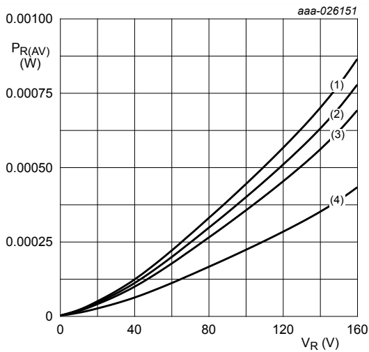
Fig. 7. Average reverse power dissipation as a function of reverse voltage; typical values T_j = 150\text{ °C} (1) \delta = 1 (2) \delta = 0.9 (3) \delta = 0.8 (4) \delta = 0.5
