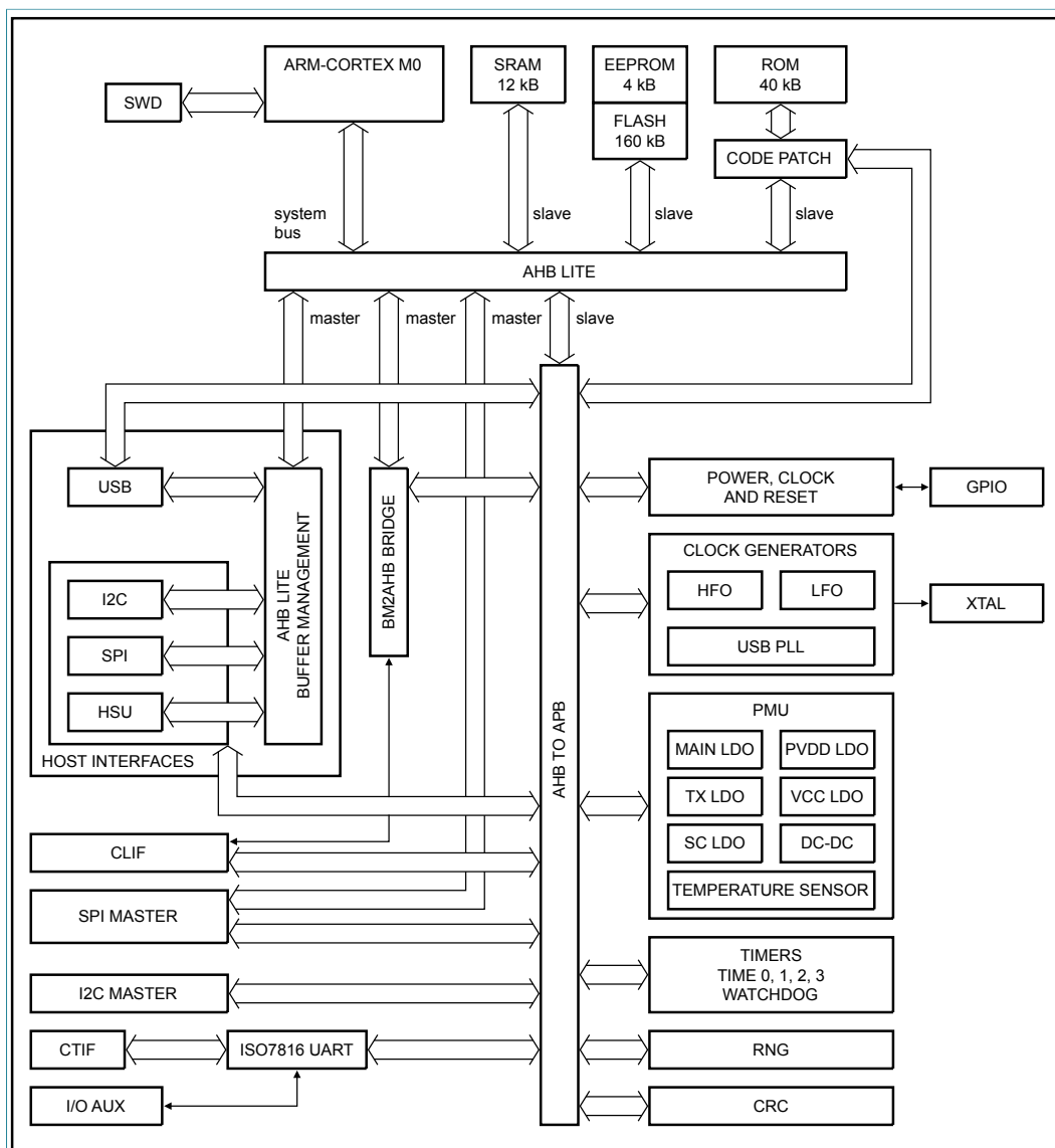
Figure 1. Block diagram
