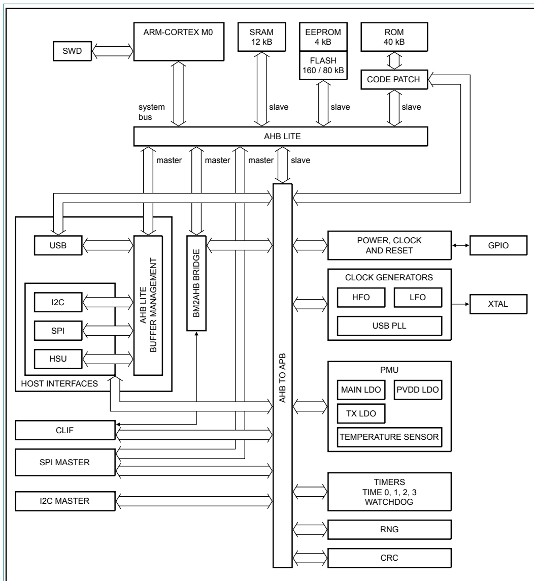
Figure 4. Block diagram
