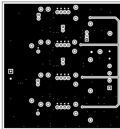
Figure 9. Bottom Layer
