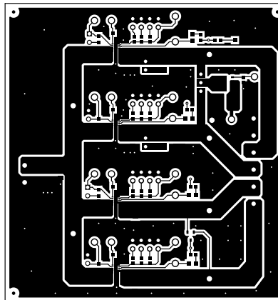
Figure 8. Top Layer
