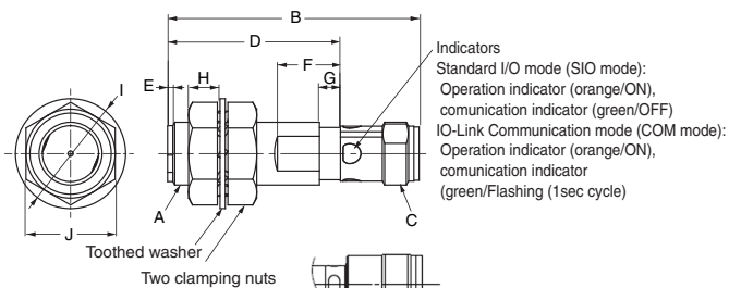
Model E2E(Q)-X□8-M1; Shape of connection.
