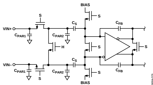
Figure 35. Switched Capacitor Input
