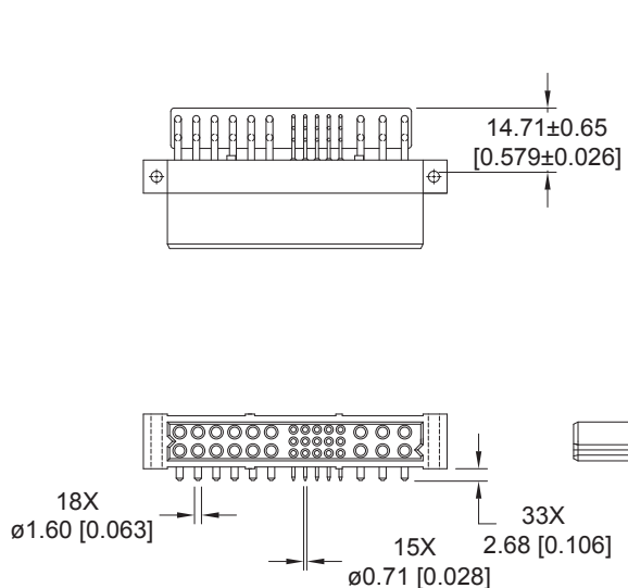
CONNECTOR DIMENSIONS
