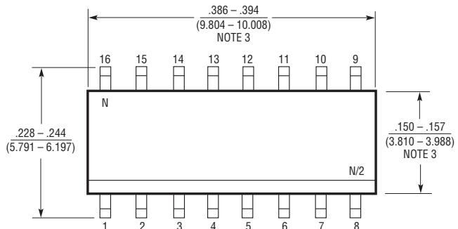
S Package 16-Lead Plastic Small Outline (Narrow .150 Inch) (Reference LTC DWG # 05-08-1610 Rev G)
