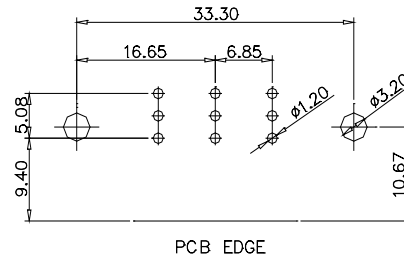
CODE:3W3/3WK3 MALE/FEMALE
