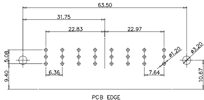
CODE:8W8 FEMALE
