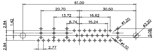
CODE:36W4 MALE
