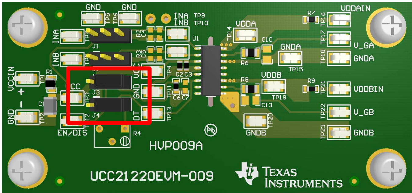
Figure 1. Jumpers Installation Position
