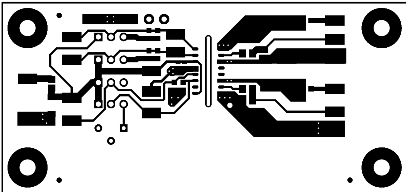
Figure 7. Top Layer
