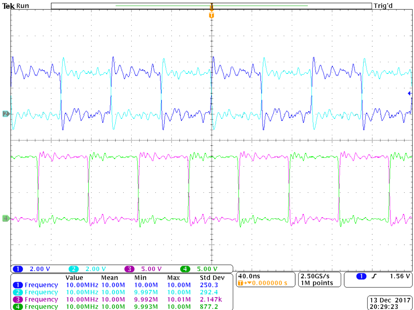
Figure 3. Example Input and Output Waveforms (Inputs: CH1 and CH2, Outputs: CH3 and CH4)
