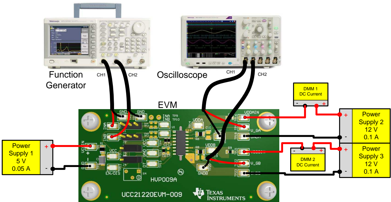
Figure 2. Bench Setup Diagram and Configuration
