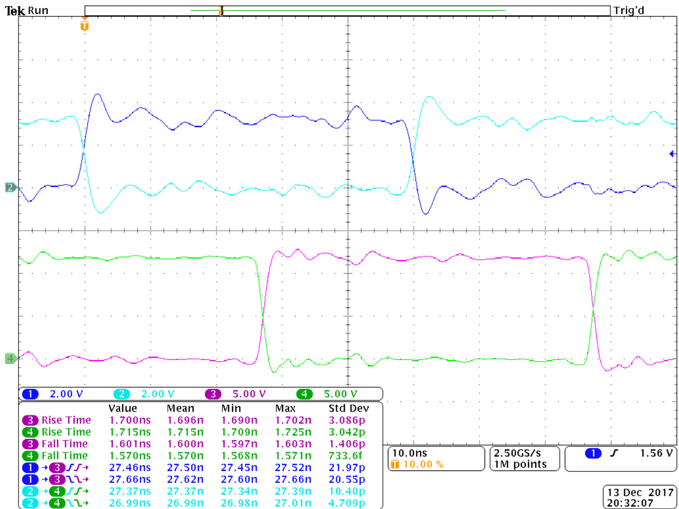
Figure 4. Example Input and Output Waveforms, Zoom In (Inputs: CH1 and CH2, Outputs: CH3 and CH4)
