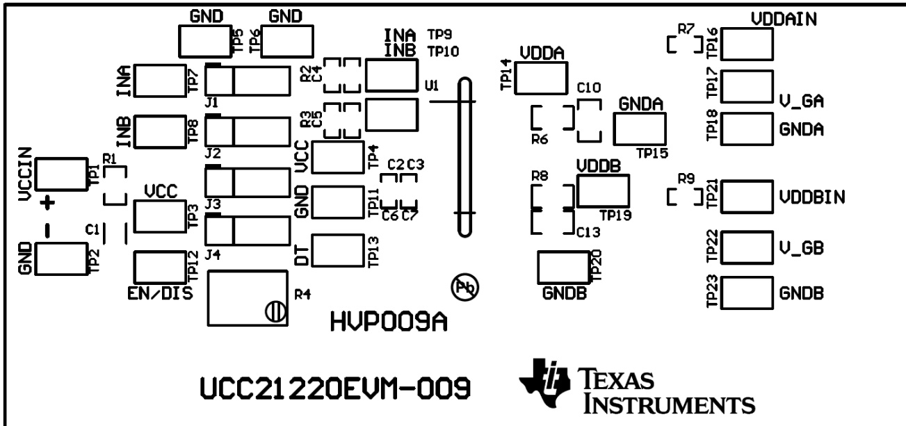
Figure 6. Top Overlay
