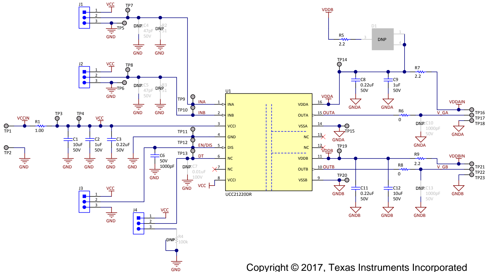
Figure 5. UCC21220EV-009 Schematic
