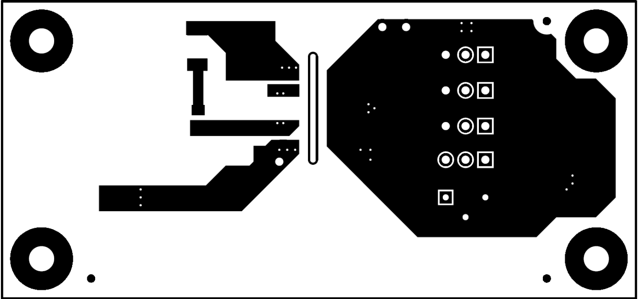
Figure 8. Bottom Layer (Flipped)
