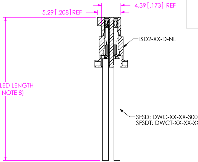
FIG 1 S2SDX-05-24-X-XX.XX-S SHOWN
