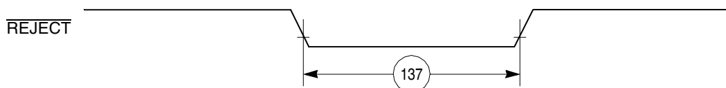
Figure 64. CAM Interface REJECT Timing Diagram
