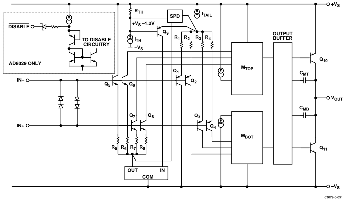
Figure 50. Simplified Schematic
