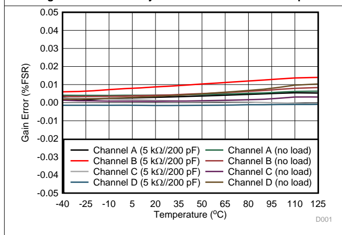
Figure 13. Gain Error vs Temperature
