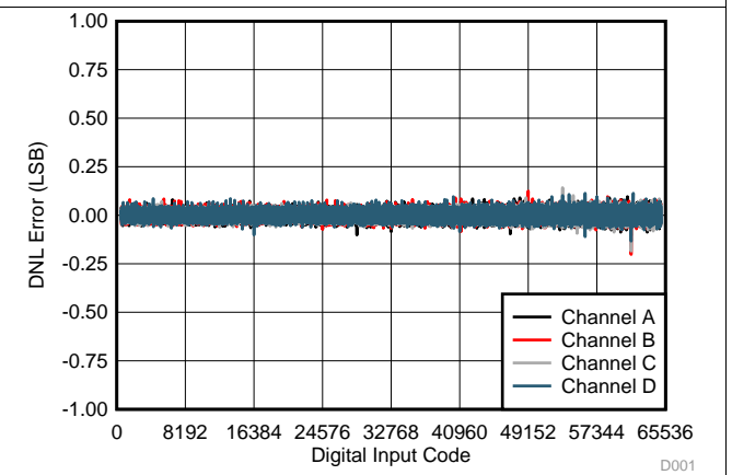
Figure 4. Differential Linearity Error vs Digital Input Code
