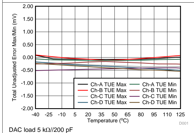
Figure 11. Total Unadjusted Error Max/Min vs Temperature
