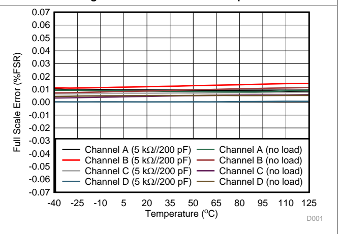
Figure 14. Full Scale Error vs Temperature
