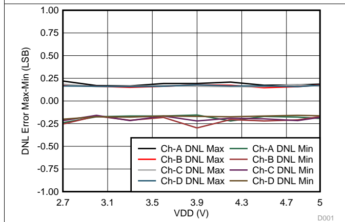
Figure 25. Differential Linearity Error (Max-Min) vs Power Supply Voltage
