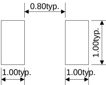
Recommended Pad Layout (mm)
