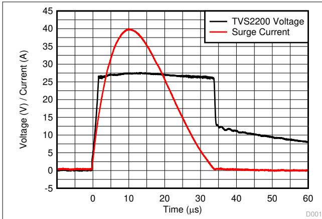
Figure 7-1. Surge Response at 40 A
