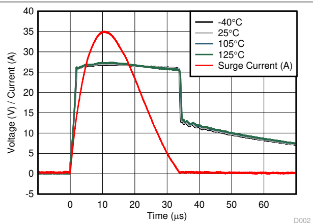
Figure 7-2. Surge Response at 35 A Across Temperature
