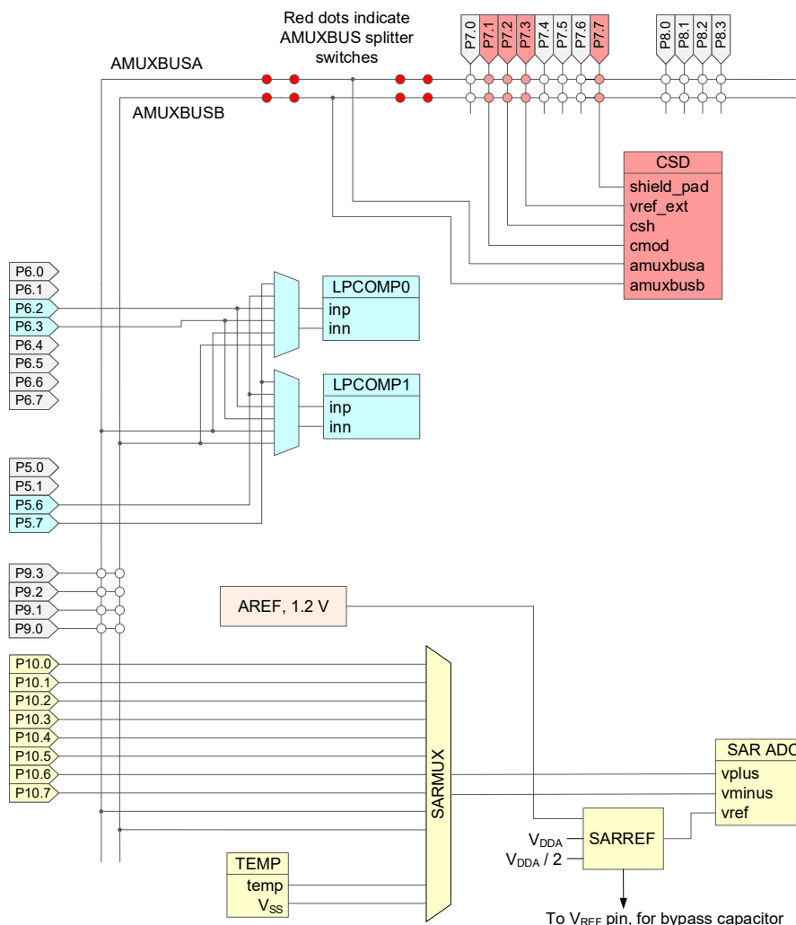
Figure 6. Analog Subsystem
