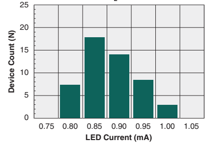
Typical I_F for Switch Dropout (N=50, I_L=300mA )
