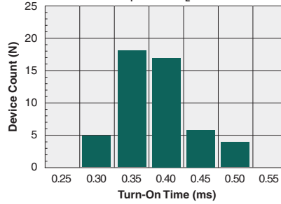
Typical Turn-On Time (N=50, I_F=5mA , I_L=300mA )
