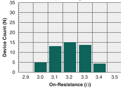
Typical On-Resistance Distribution (N=50, I_F=2mA , I_L=300mA )
