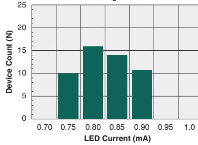
Typical I_F for Switch Operation (N=50, I_L=300mA )
