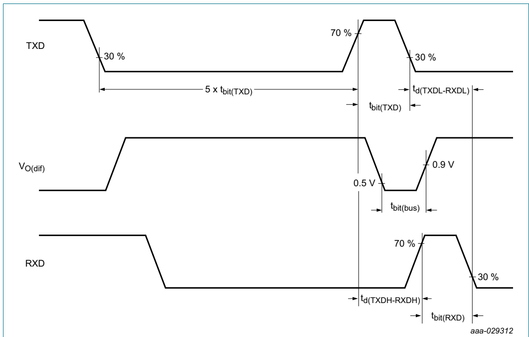
Fig 12. CAN FD timing definitions according to ISO 11898-2:2016
