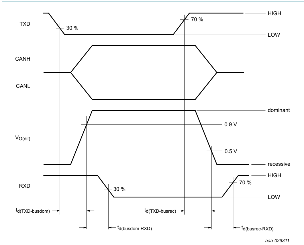
Fig 11. CAN transceiver timing diagram
