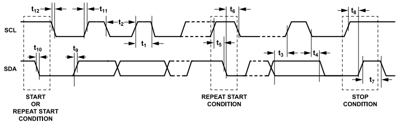
Figure 3. I 2 C Serial Interface Timing Diagram
