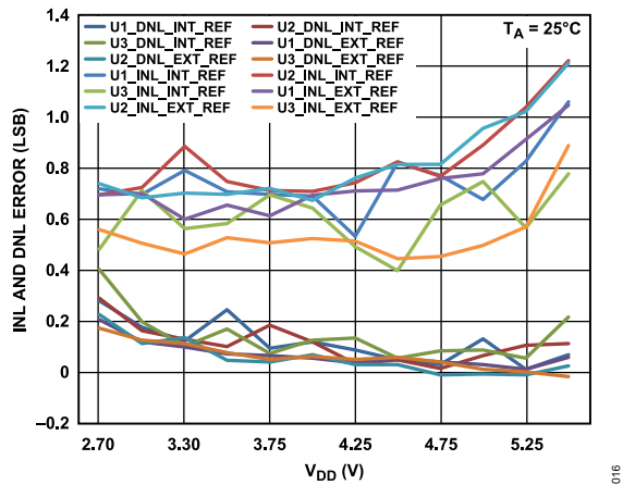
Figure 16. INL and DNL Error vs. V_{DD}
