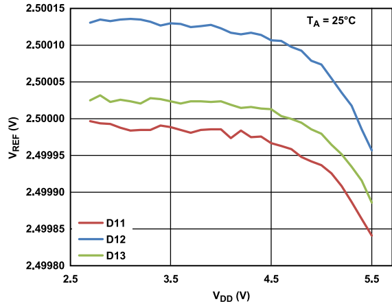
Figure 27. Internal Reference Voltage vs. V_{DD}
