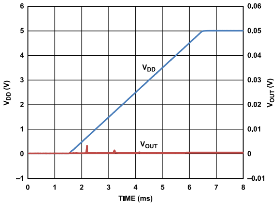
Figure 41. Power-On Reset to 0 V
