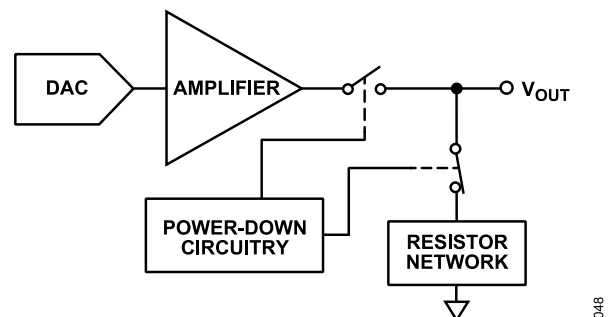
Figure 48. Output Stage During Power-Down
