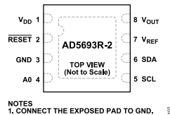
Figure 8. AD5693R-2 Pin Configuration, 8-Lead LFCSP, \overline{\text{RESET}} Option
