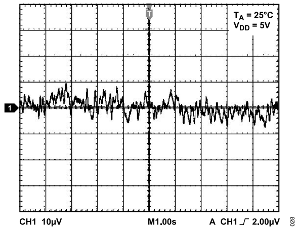
Figure 28. Internal Reference Noise, 0.1 Hz to 10 Hz
