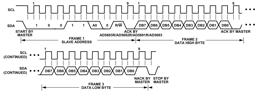
Figure 49. I 2 C Read Operation
