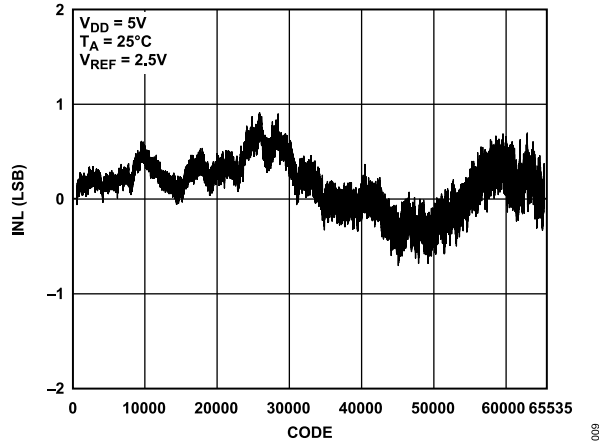
Figure 9. AD5693R/AD5693 INL
