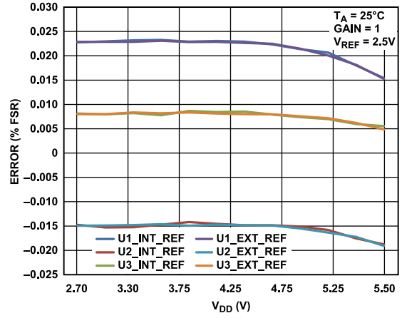
Figure 24. Gain Error and Full-Scale Error vs. V DD
