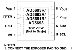
Figure 6. AD5693R/AD5692R/AD5691R/AD5693 Pin Configuration, 8-Lead LFCSP, LDAC Option
