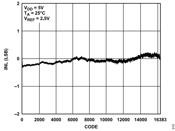
Figure 10. AD5692R INL
