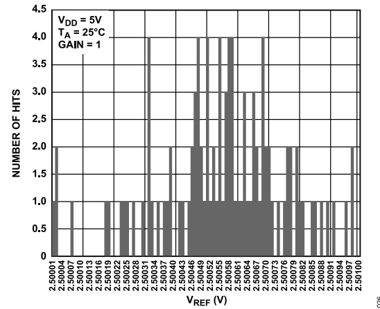
Figure 26. Reference Output Spread
