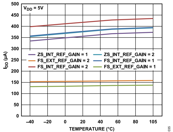
Figure 35. I_{DD} vs. Temperature
