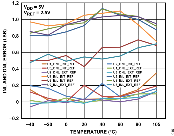
Figure 15. INL and DNL Error vs. Temperature (AD5693R/AD5693)
