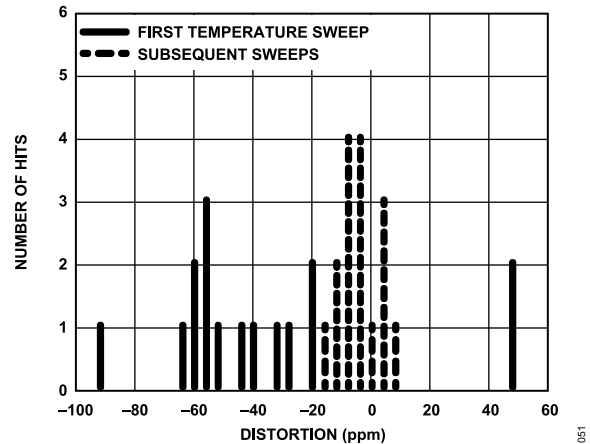
Figure 50. Thermal Hysteresis
