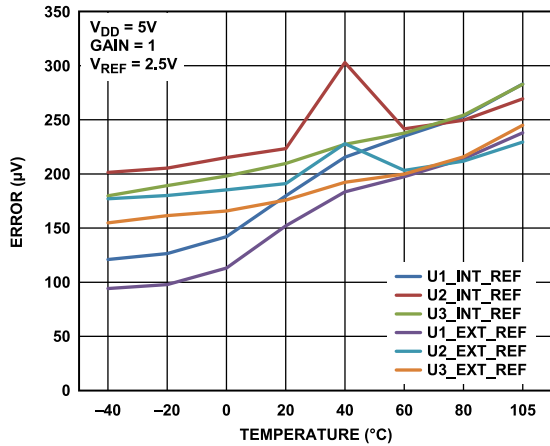
Figure 22. Zero Code Error and Offset Error vs. Temperature
