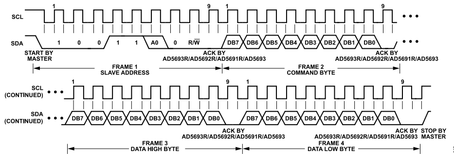
Figure 47. I 2 C Write Operation
