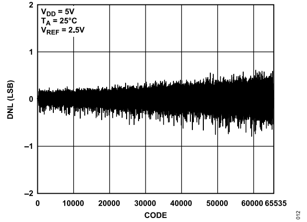
Figure 12. AD5693R/AD5693 DNL
