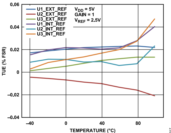
Figure 17. TUE vs. Temperature
