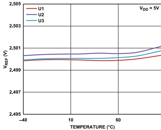
Figure 23. Internal Reference Voltage vs. Temperature (Grade B)
