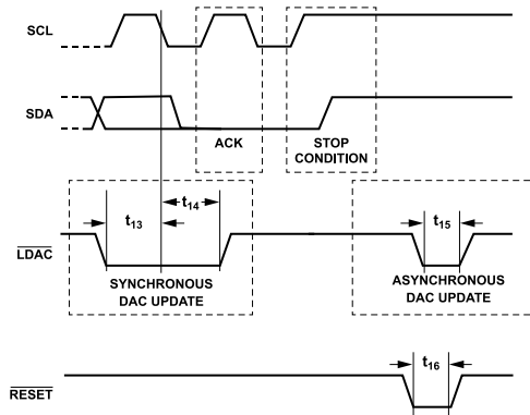
Figure 4. I 2 C RESET and LDAC Timing
