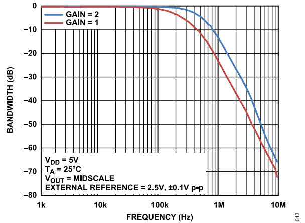
Figure 43. Multiplying Bandwidth, External Reference = 2.5 V, ±0.1 V p-p, 10 kHz to 10 MHz
