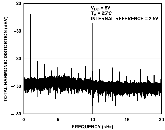
Figure 40. Total Harmonic Distortion at 1 kHz
