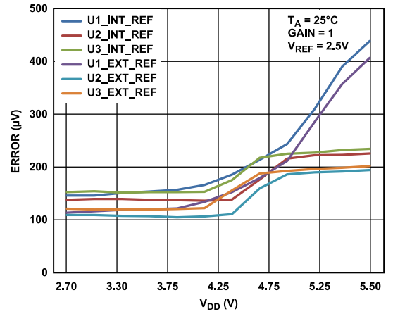
Figure 25. Zero Code Error and Offset Error vs. V DD
