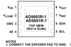
Figure 7. AD5693R-1/AD5691R-1 Pin Configuration, 8-Lead LFCSP, V_{\text{LOGIC}} Option
