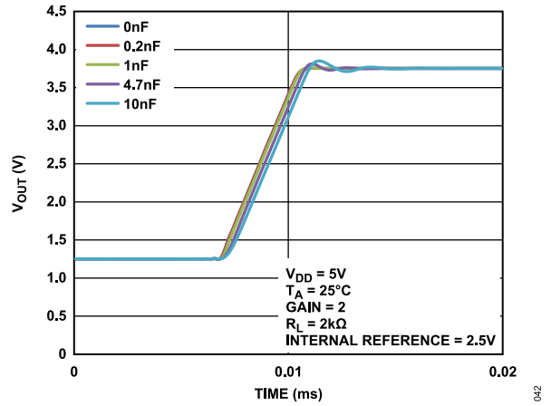
Figure 42. Capacitive Load vs. Settling Time, Gain = 2
