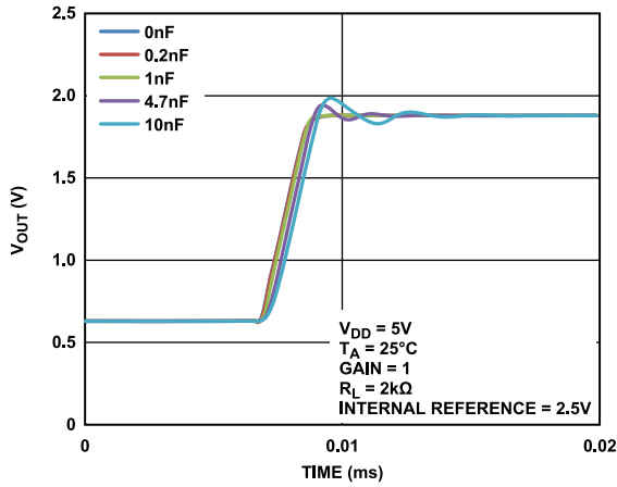
Figure 39. Capacitive Load vs. Settling Time, Gain = 1
