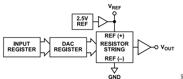
Figure 45. DAC Channel Architecture Block Diagram
