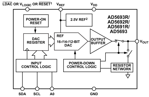
Figure 1. MSOP
