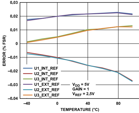
Figure 21. Gain Error and Full-Scale Error vs. Temperature
