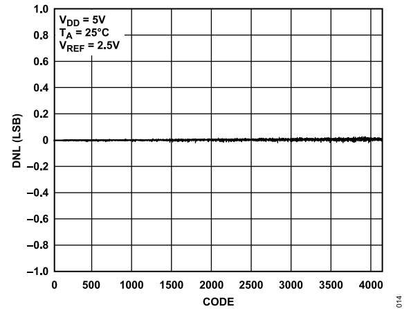
Figure 14. AD5691R DNL
