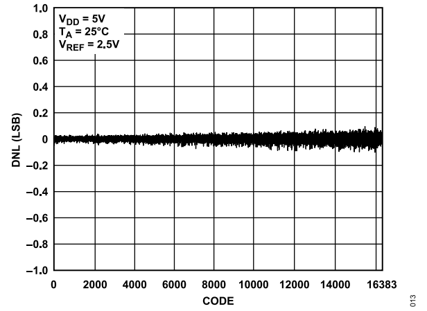
Figure 13. AD5692R DNL
