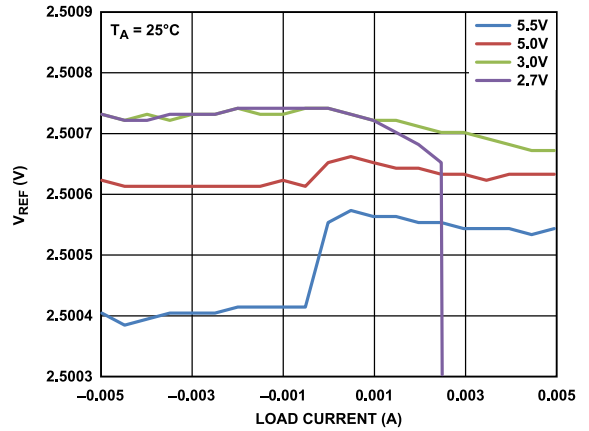
Figure 30. Internal Reference Voltage vs. Load Current
