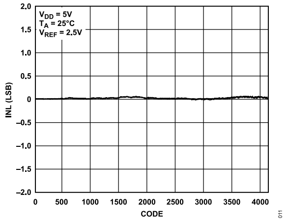
Figure 11. AD5691R INL
