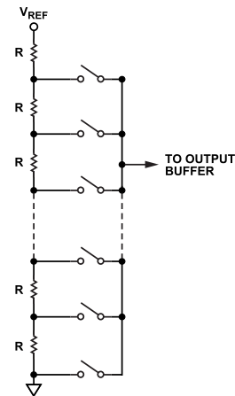
Figure 46. Simplified Resistor String Structure
