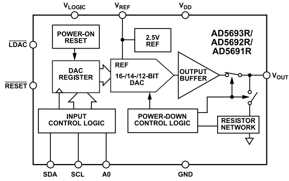
Figure 1. MSOP
