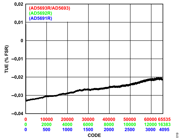
Figure 19. TUE vs. Code
