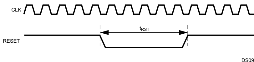
Figure 30-3. Non-Power-On Reset
