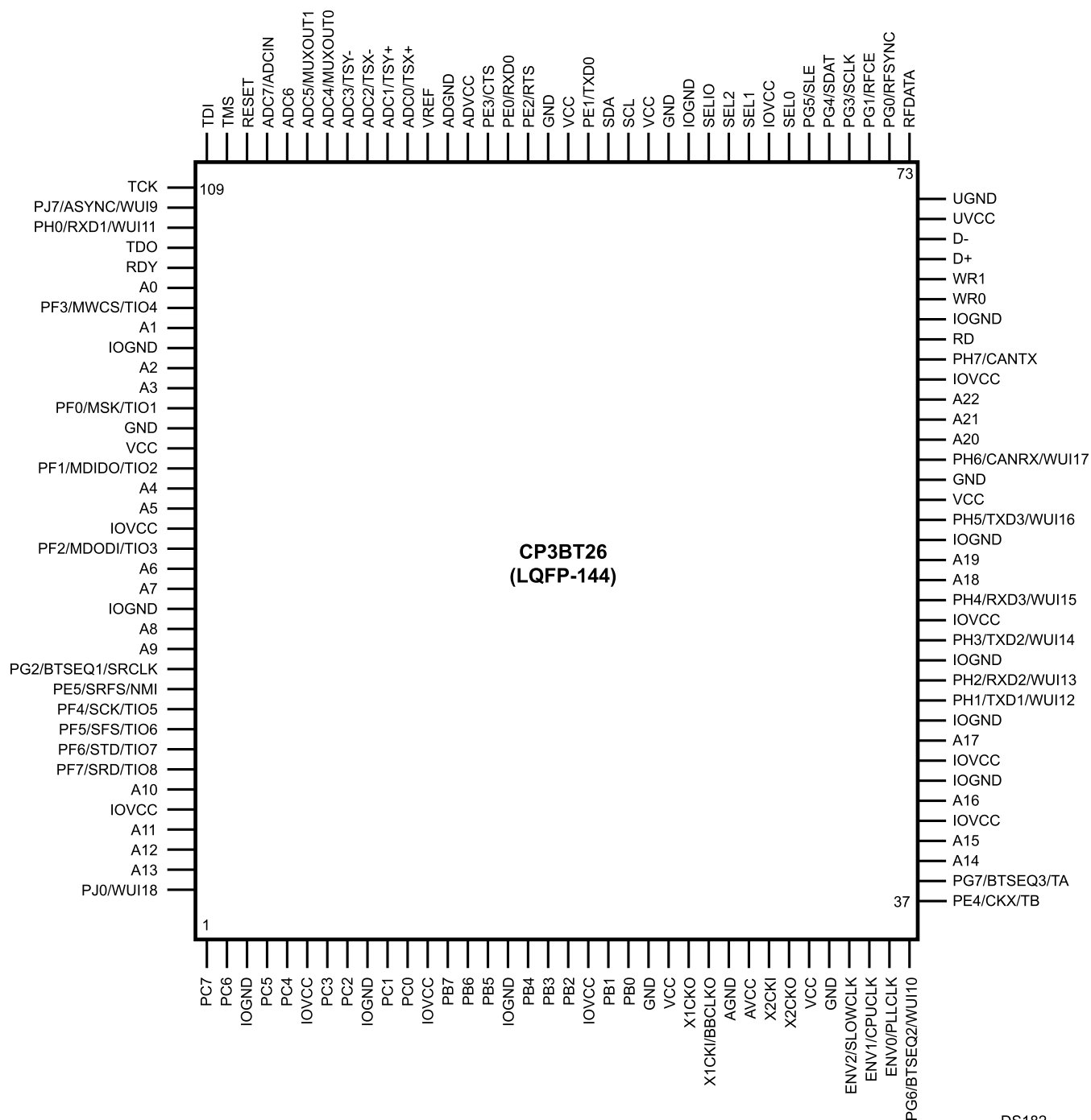
Figure 31-2. CP3BT26 in the LQFP-144 Package (Top View)
