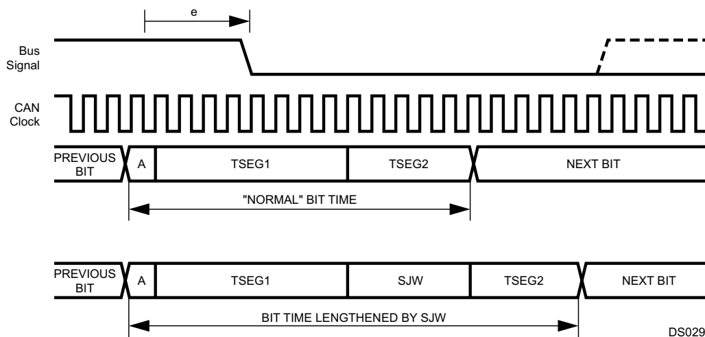
Figure 19-12. Resynchronization ( e > SJW )
