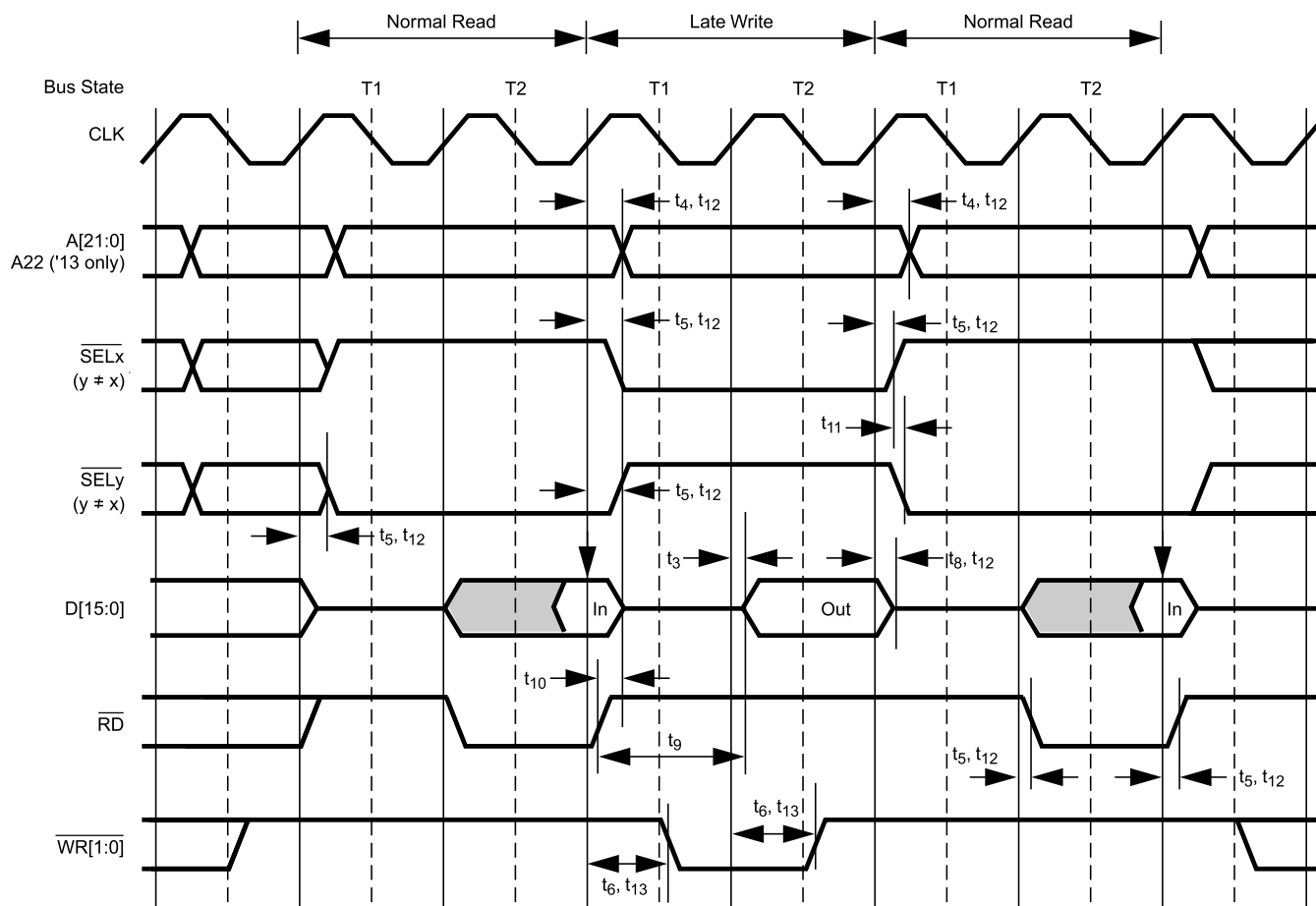
Figure 30-23. Late Write Between Normal Read Cycles (No Wait States)
