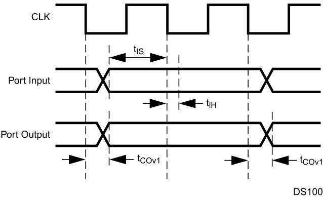
Figure 30-6. I/O Port Timing
