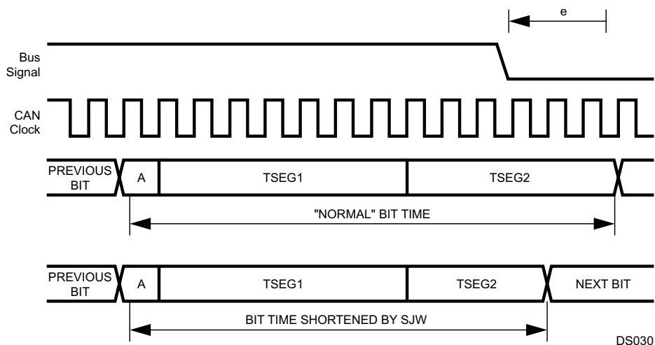
Figure 19-13. Resynchronization ( e < -SJW )
