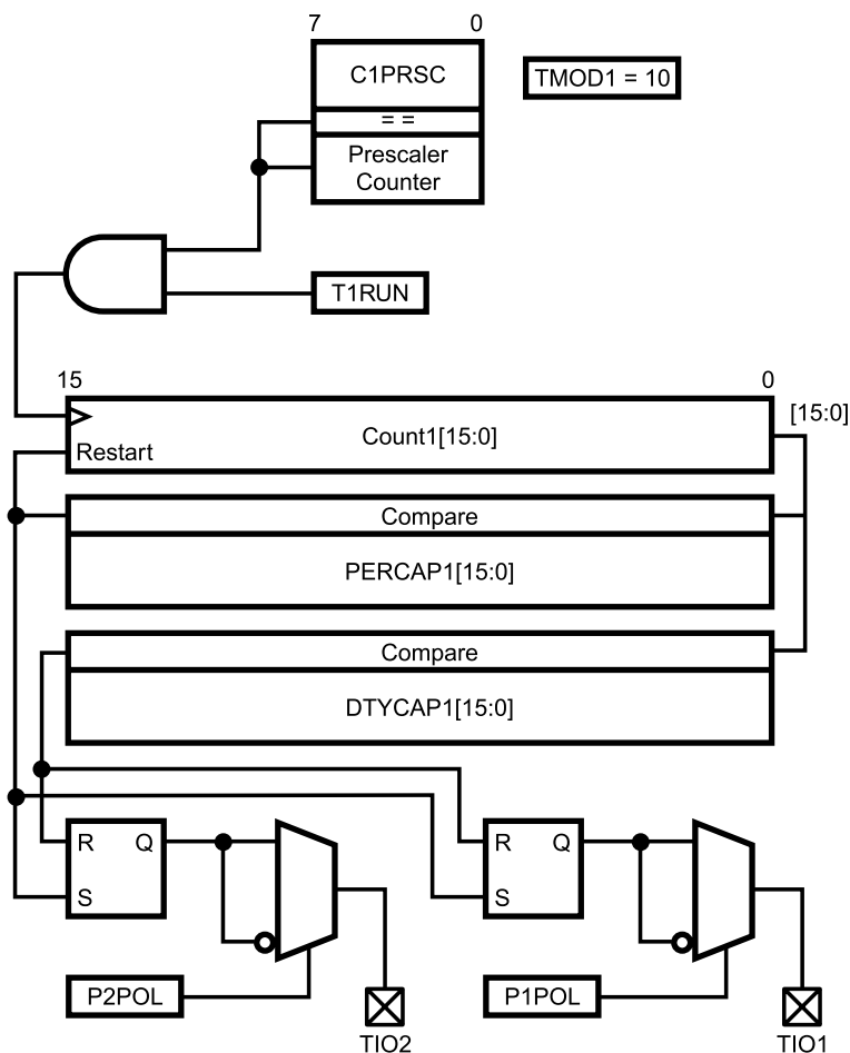
Figure 27-4. VTU 16-bit PWM Mode
