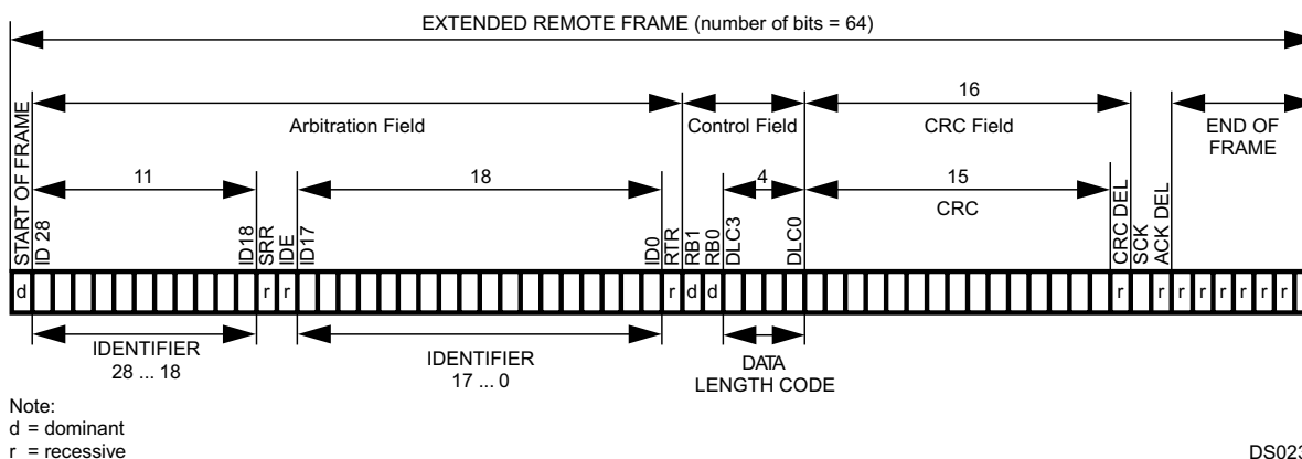
Figure 19-6. Extended Remote Frame
