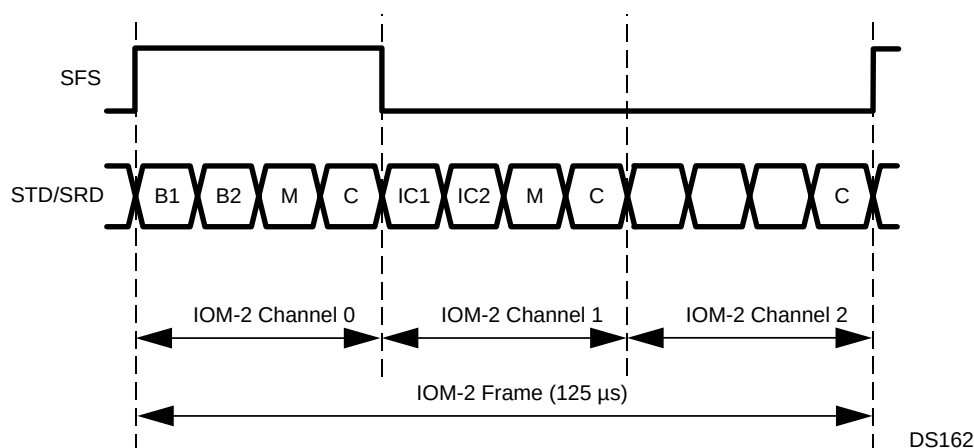
Figure 20-9. IOM-2 Frame Structure
