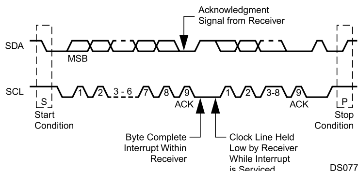
Figure 24-3. ACCESS.bus Data Transaction
