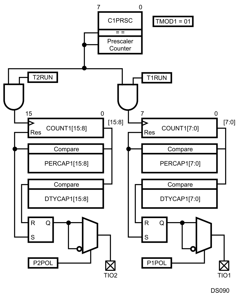
Figure 27-3. VTU Dual 8-Bit PWM Mode
