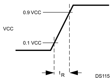
Figure 30-4. Power-On Reset
