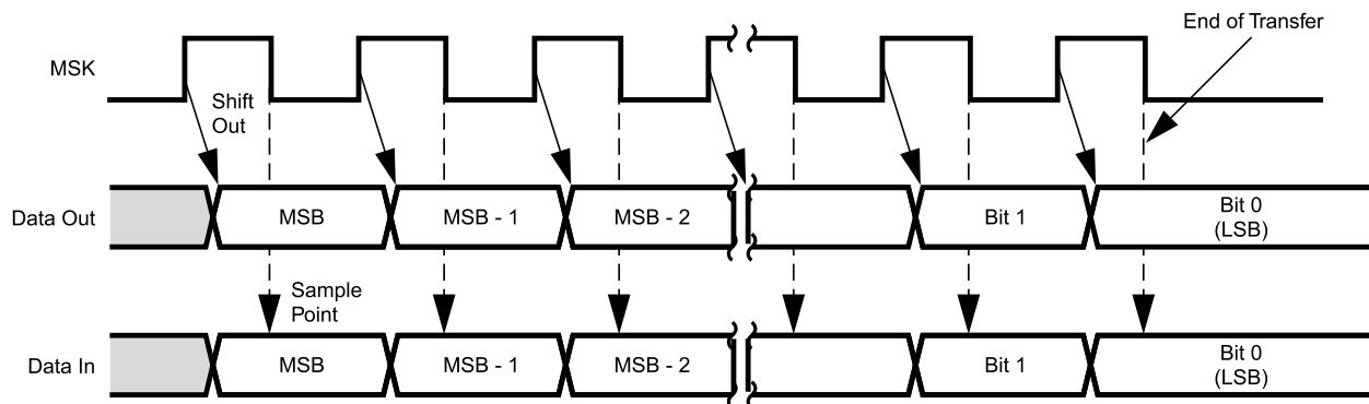
Figure 23-5. Alternate Mode (SCIDL = 0)
