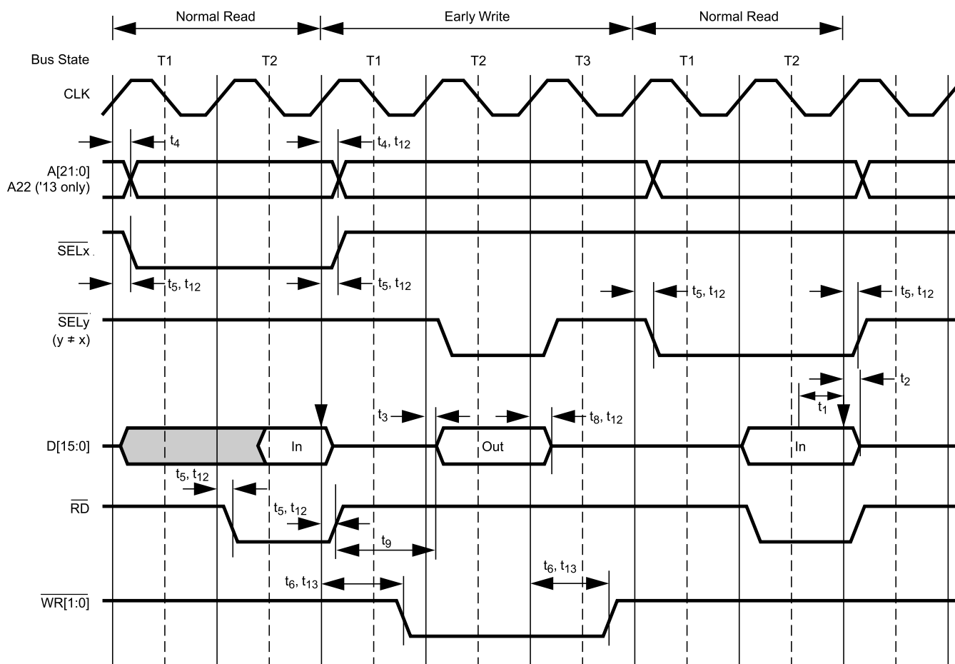
Figure 30-22. Early Write Between Normal Read Cycles (No Wait States)
