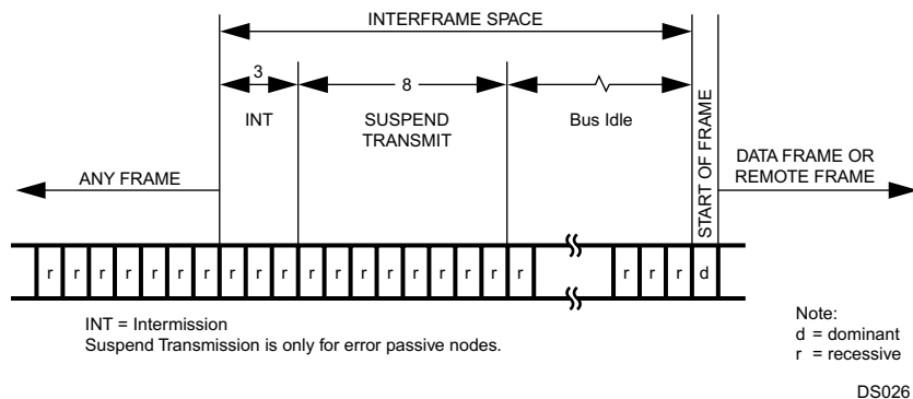
Figure 19-9. Interframe Space
