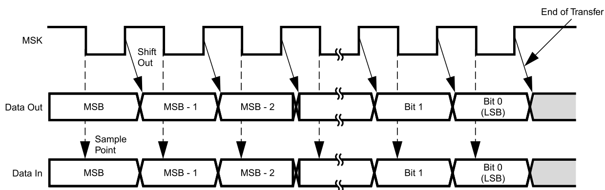
Figure 23-5. Alternate Mode (SCIDL = 0)
