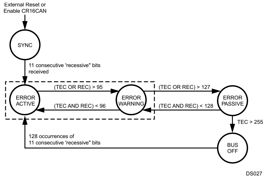
Figure 19-10. Bus States
