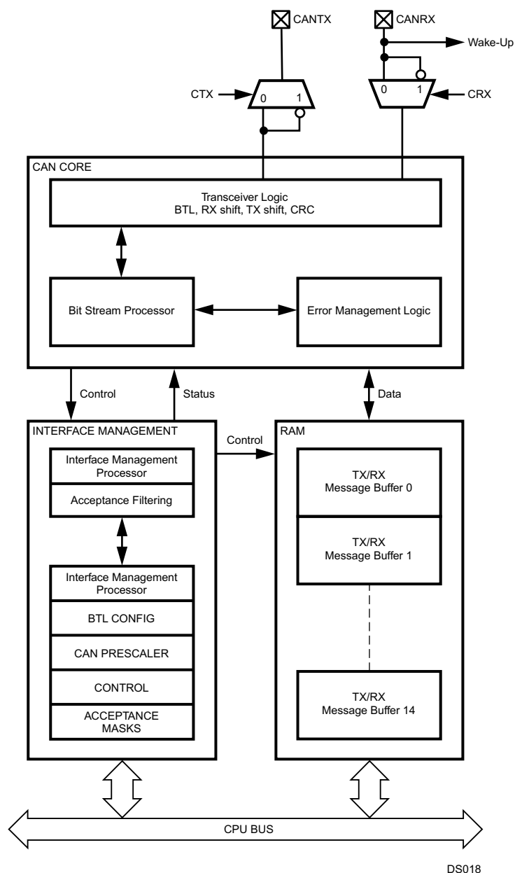
Figure 19-1. CAN Block Diagram
