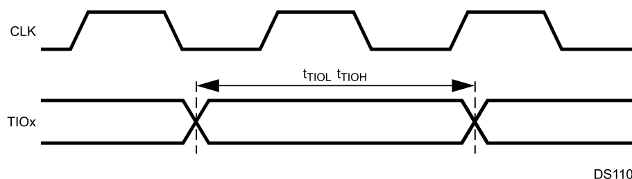
Figure 30-21. Versatile Timing Unit Input Timing
