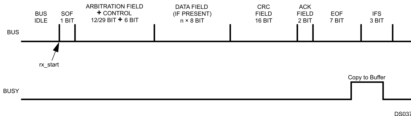
Figure 19-20. Receive Timing
