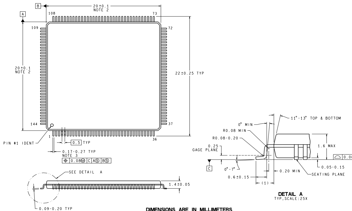
Figure 32-2. LQFP-144 Package
