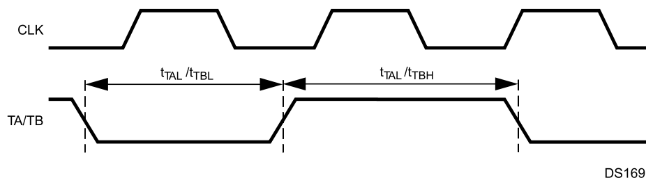
Figure 30-20. Multi-Function Timer Input Timing
