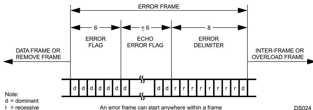
Figure 19-7. Error Frame
