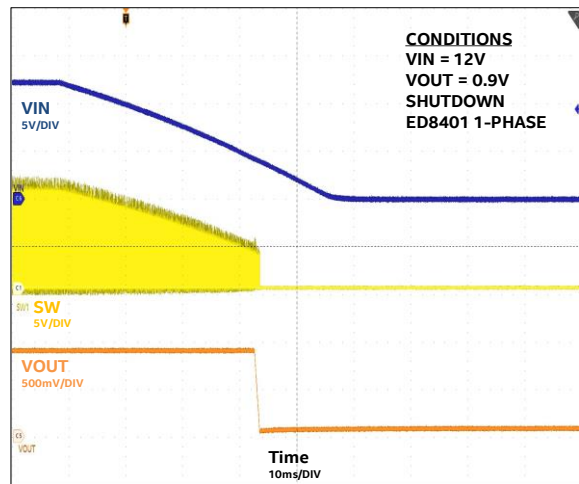
Shutdown with VIN at No Load (1-Phase)
