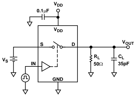
Figure 23. Switching Times
