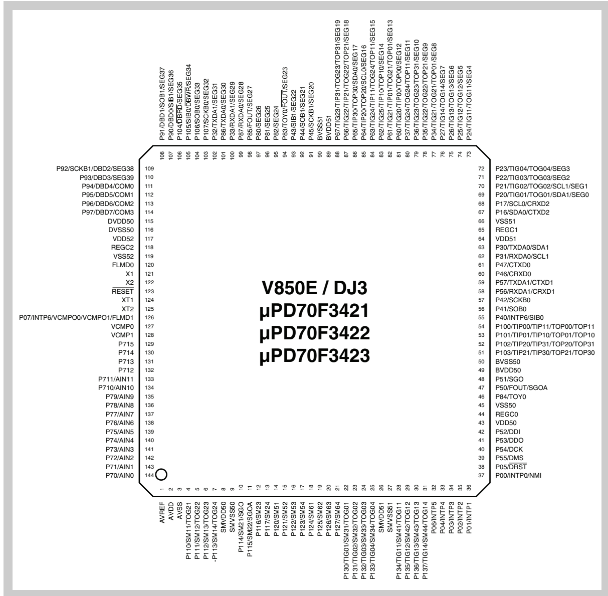
Figure 2-3 Pin Configuration μPD70F3423, μPD70F3422, μPD70F3421
