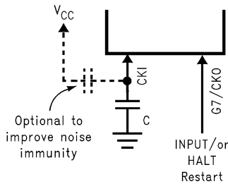
Figure 22. External Oscillator
