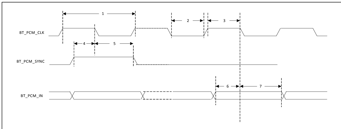
Figure 12. PCM Burst Mode Timing (Receive Only, Short Frame Sync)
