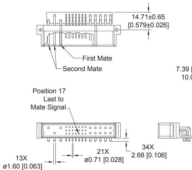
CONNECTOR DIMENSIONS
