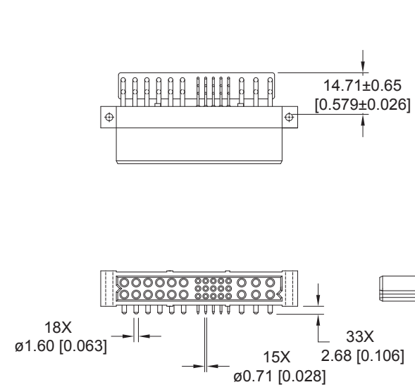
CONNECTOR DIMENSIONS
