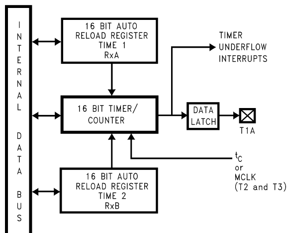
Figure 17. Timer in PWM Mode
