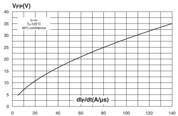
Figure 12: Transient peak forward voltage versus di_F/dt (damper diode)
