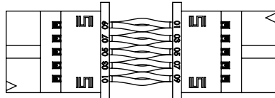
FIG 3 T2SDX-05-28-X-XX.XX-D-NUX SHOWN (SAME AS FIG 1 EXCEPT AS SHOWN) (PIN 01 TO N)
