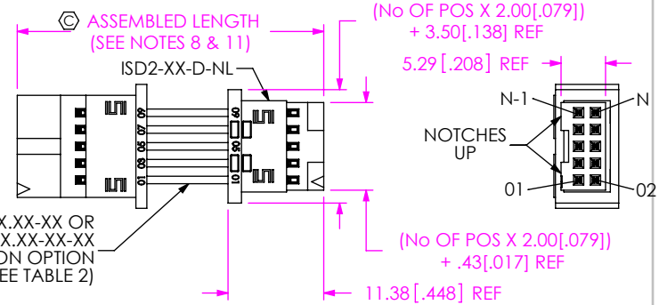
FIG 6 T2SDX-05-28-X-XX.XX-T-NUS SHOWN (SAME AS FIG 1 EXCEPT AS SHOWN) (PIN 01 TO 01)
