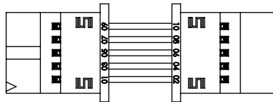
FIG 4 T2SDX-05-28-X-XX.XX-D-NDS SHOWN (SAME AS FIG 1 EXCEPT AS SHOWN) (PIN 01 TO 02)
