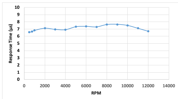
Figure 19: Measured Response Time Over RPM
