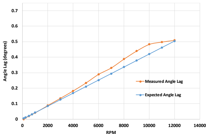
Figure 18: Measured Angle Lag vs. RPM
