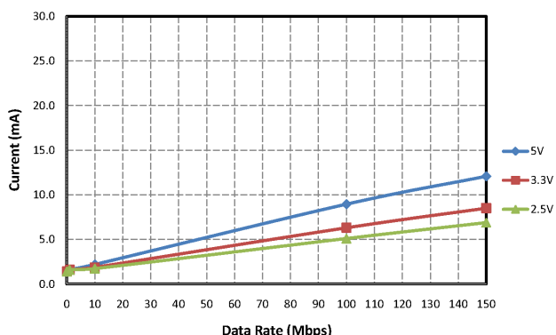
Figure 8. Si8620 Typical V_{DD2} Supply Current vs. Data Rate 5, 3.3, and 2.50 V Operation (15 pF Load)
