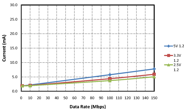
Figure 9. Si8621 Typical V_{DD1} or V_{DD2} Supply Current vs. Data Rate 5, 3.3, and 2.50 V Operation (15 pF Load)
