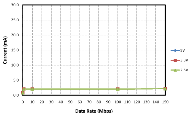
Figure 7. Si8620 Typical V_{DD1} Supply Current vs. Data Rate 5, 3.3, and 2.50 V Operation
