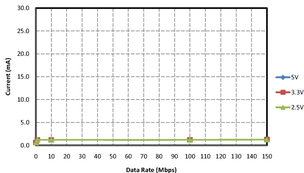
Figure 5. Si8610 Typical V_{DD1} Supply Current vs. Data Rate 5, 3.3, and 2.50 V Operation
