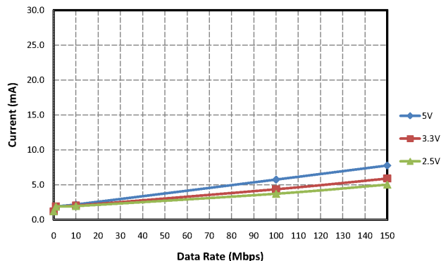
Figure 10. Si8622 Typical V_{DD1} or V_{DD2} Supply Current vs. Data Rate 5, 3.3, and 2.50 V Operation (15 pF Load)
